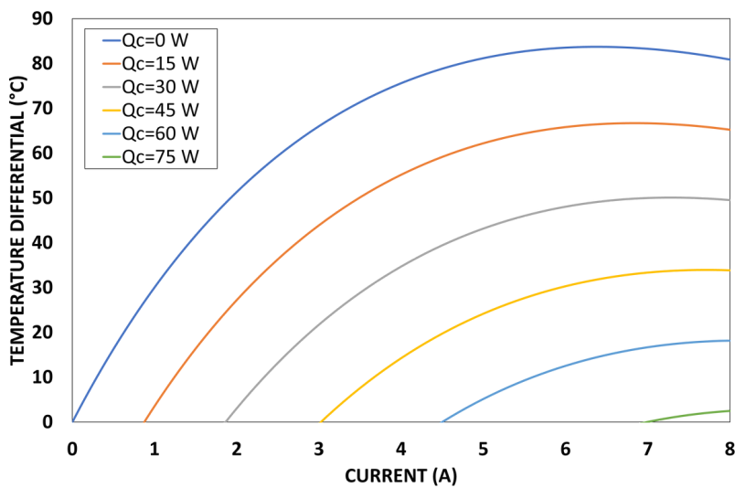
Current vs. Temperature Differential
